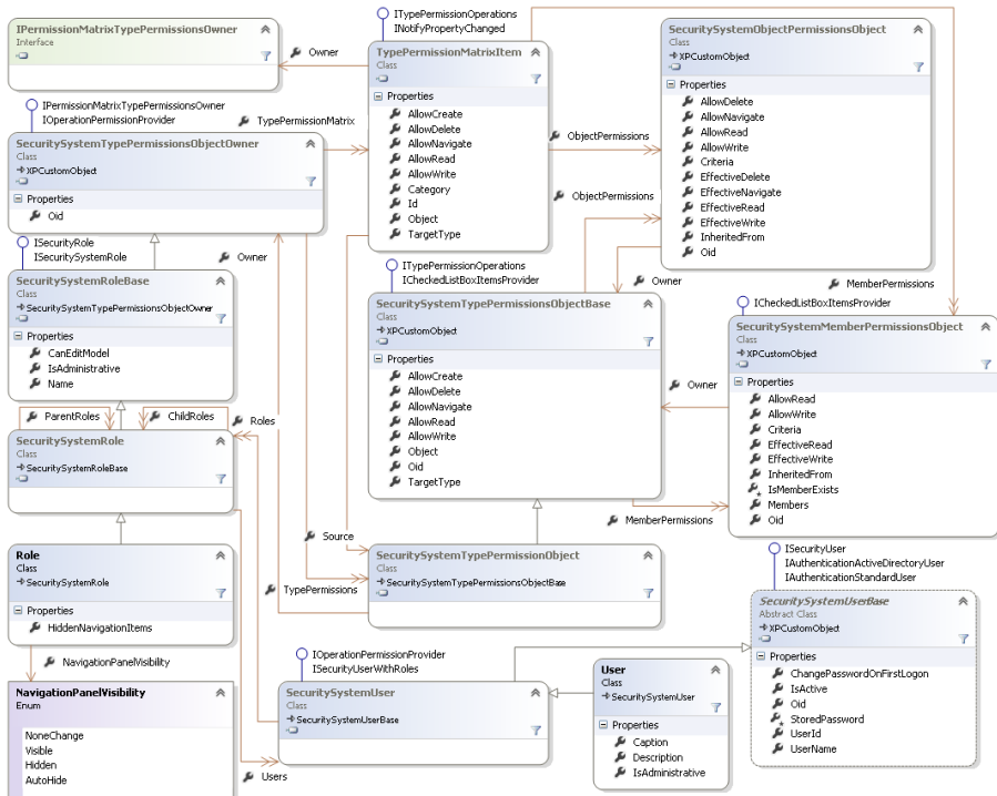
Fig. 3. UML class diagram of the implemented model of access rights differentiation
