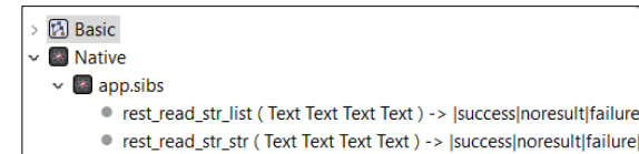
Fig. 2. SIBs explorer with the new Native SIBs
