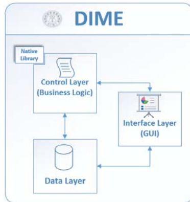
Fig. 1. DIME: Modelling Architecture and Native Library support
