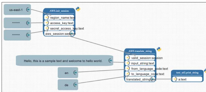
Fig. 5. Pyrus pipeline using AWS translate
