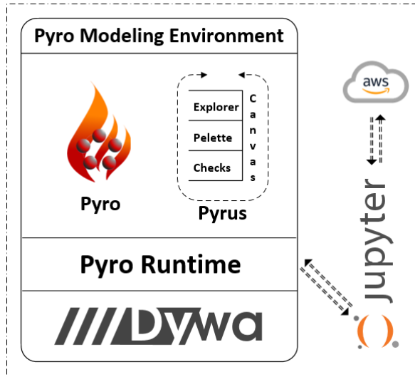
Fig. 4. The Pyrus/Pyro Architecture extended with AWS
