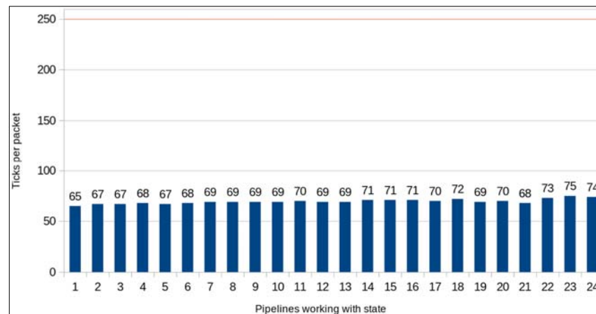
Fig. 2 Shared bus approach evaluation results
