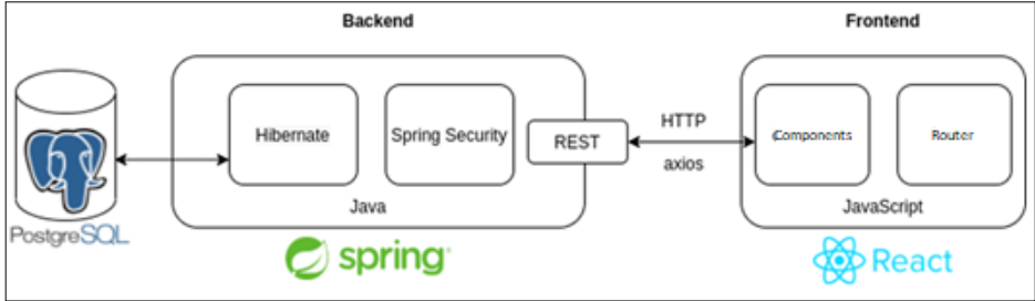
Fig. 2. Software architecture
