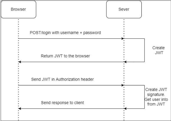
Fig. 3. JWT authorization scheme
