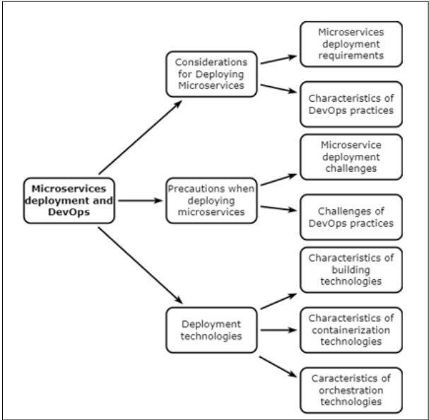
Fig. 3. Meta-aggregation classification
