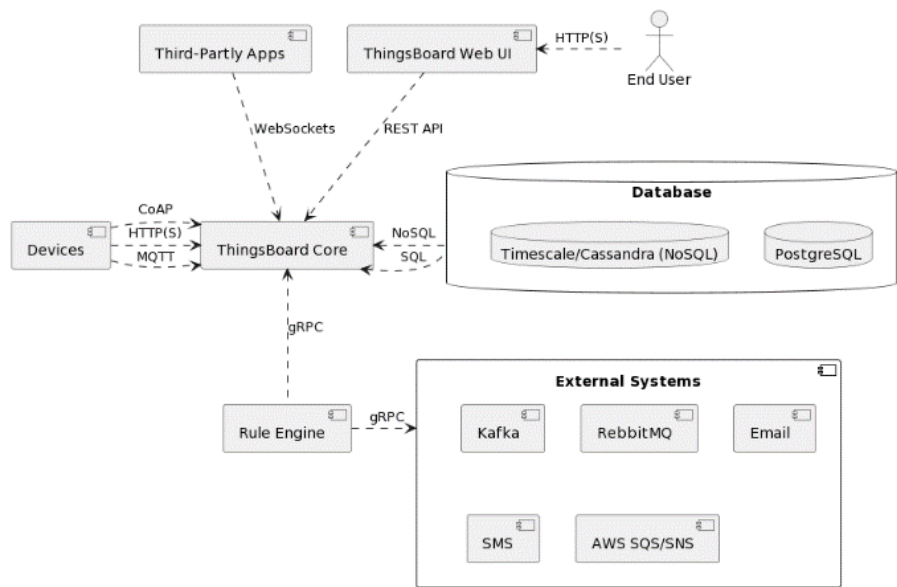
Fig.2. Component diagram for monolithic architecture of ThingsBoard
