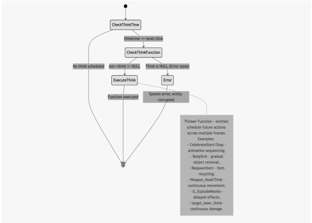
Fig. 2. Main loop ( G_RunFrame() ) statechart.
