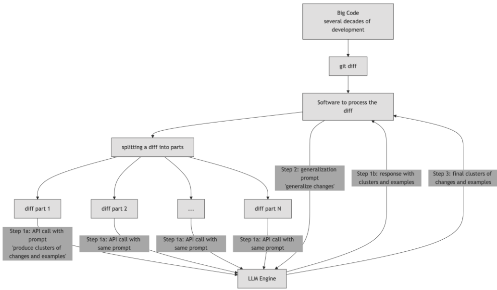
Fig. 4. LLM-driven diff analysis.
