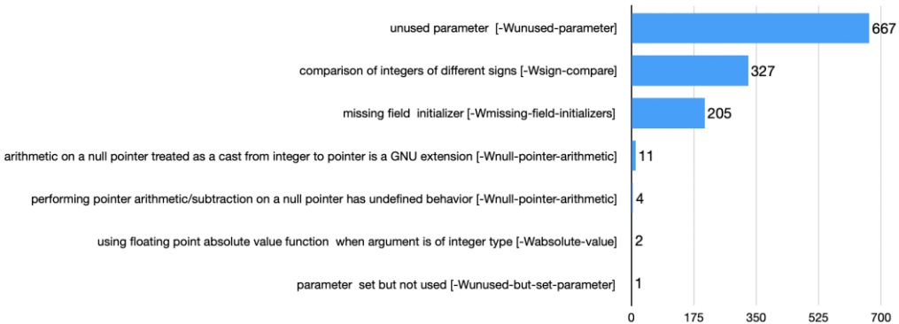
Fig. 5. GCC warnings classification in the ioquake3 project.
