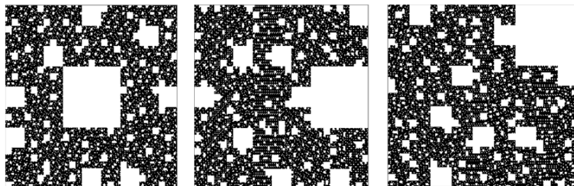
Fig.7. Three types of Random Sierpinski Carpets with five size levels of recurrence. They represent possible levels of Health Centers in an urban area. In spite of their different Networks, the spatial Fractal dimension D = \log 8 / \log 3 = 1.8928 is the same but in a statistical sense [13, 14]
