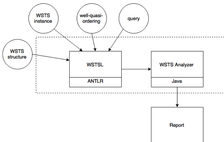
Fig. 1. Architecture of the developed tool
