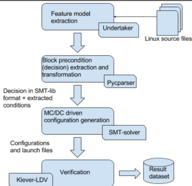
Fig. 2. OStap workflow.
