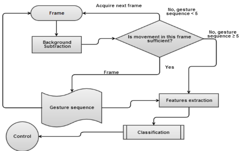
Fig. 1. The workflow of the algorithm.
