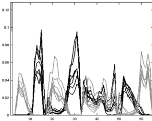
Fig. 4. Plot of 14 histograms containing samples from two classes: "hand up" and "hand down". Black colour corresponds to "hands down" movement, gray colour corresponds to "hands up" movement. Feature vector element numbers displayed on horizontal axis and values on vertical axis.
